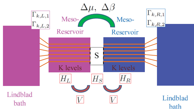
FIG. 1. (Color online) Schematic view of the two-level reservoir open-system model.
