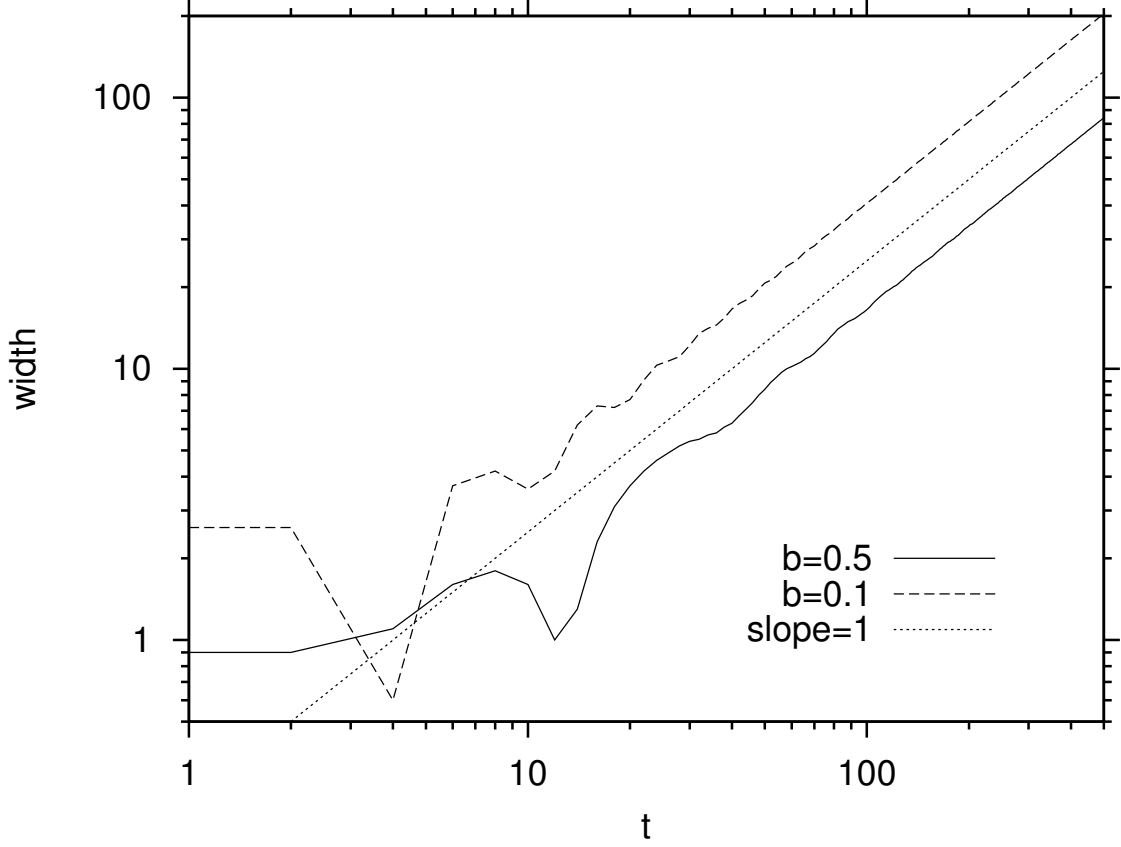
FIG. 2. The width, \sigma(t) \equiv \sqrt{(\sum_n n^2 h_n)/(\sum_n h_n)} , of a pulse spreading from an initial single-site disturbance as a function of time in the IKSG model for two different values of parameter b = \tan \delta . The initial excitation is delta-like with \phi_0^+ = 2, \phi_0^- = 3, \phi_n^\pm = 0, n \neq 0 . A finite lattice of length N = 800 with periodic boundary conditions has been used in the simulation. The line with slope 1 is used to guide the eye: the figure provides clear evidence of ballistic transport, \sigma(t) \sim t .
