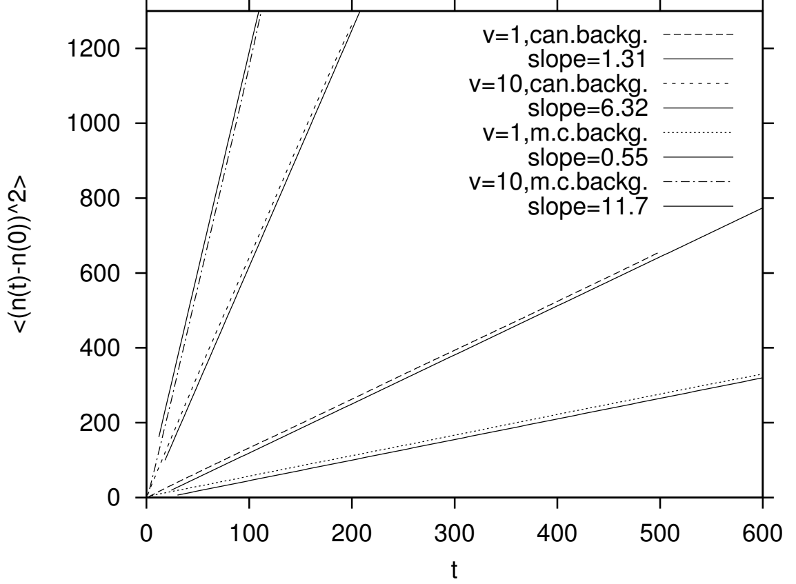
FIG. 17. Diffusion of ‘velocitons’ in MNC-PIBB lattice. We show root-mean-square displacements vs. time for velocitons with v = 1 and v = 10 , in either canonically thermalized background with temperature T = 1 or in ‘microcanonically thermalized’ background (all background particles have equal unit velocities but random signs and initial positions). Full lines give the slopes of best linear fits which support the existence of normal diffusion.
