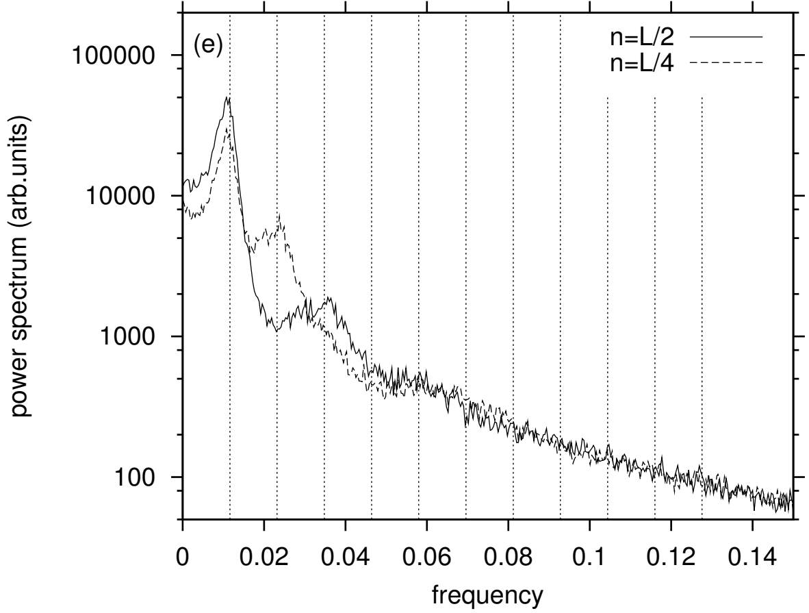
FIG. 10. Thermal excitation of acoustic modes: (a) the time dependence of the displacement q_n(t) of the particle in the middle n = L/2 of the diatomic ( m_2/m_1 = 0.382, b = 1.0 ) bing-bang lattice of size L = 400 between thermal reservoirs in equilibrium ( T_L = T_R = 1 ); (b) the power-spectrum of the same signal ( n = L/2 , full curve) and for the displacements at the one-quarter of the chain ( n = L/4 , dashed curve); dotted vertical lines denote integer multiples of the basic acoustic frequency; (c) the same plot as in (b) but for the MC-EBB with b = 2 (nonvanishing pressure); (d) the same plot as in (b) but for the MC-PIBB with b = 1 (vanishing pressure); and (e) the same plot as in (b) but for the MC-PIBB with b = 2 (non-vanishing pressure).
