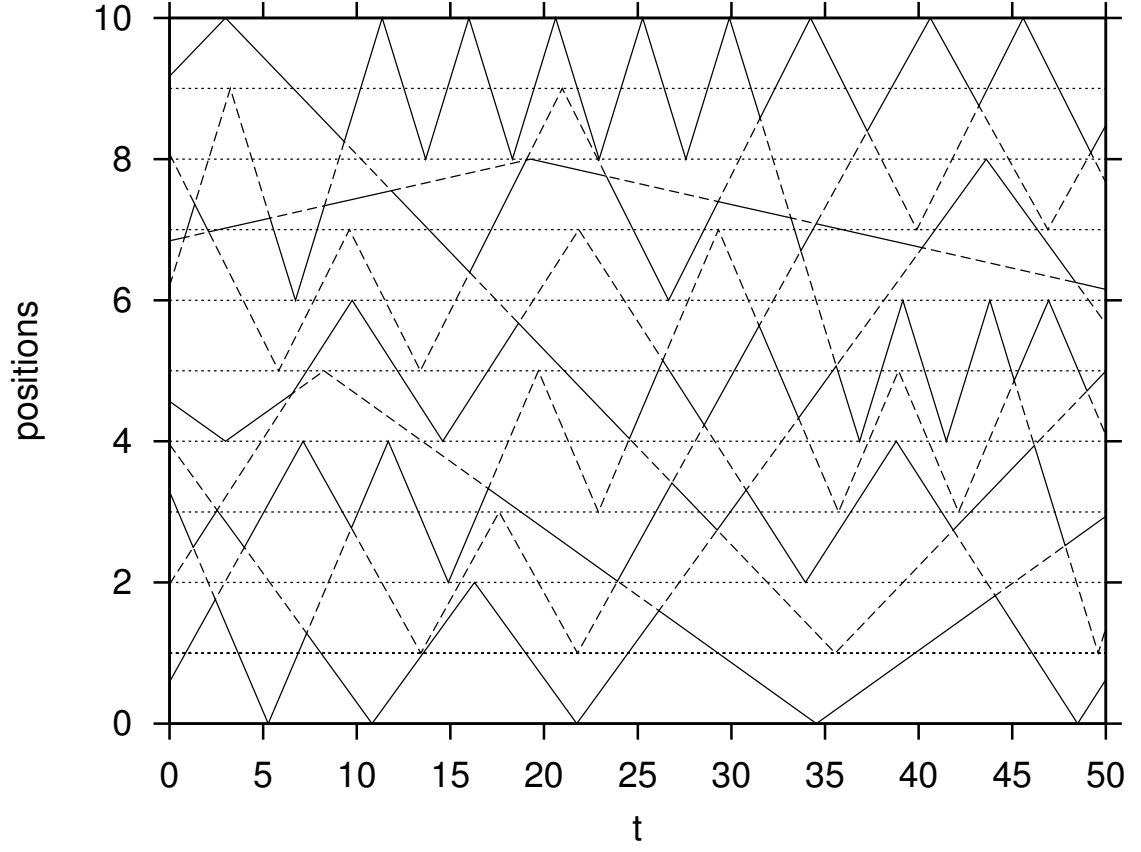
FIG. 12. A typical trajectory of MNC-PIBB chain ( L = 9 ). As in Fig.3, the ordinate shows particle positions ( x_n(t) ) where for clarity the odd n particle trajectories are plotted with full lines while the even n trajectories are dashed. The walls at x = 0 and x = 10 act as thermal baths at temperature T = 1 .
