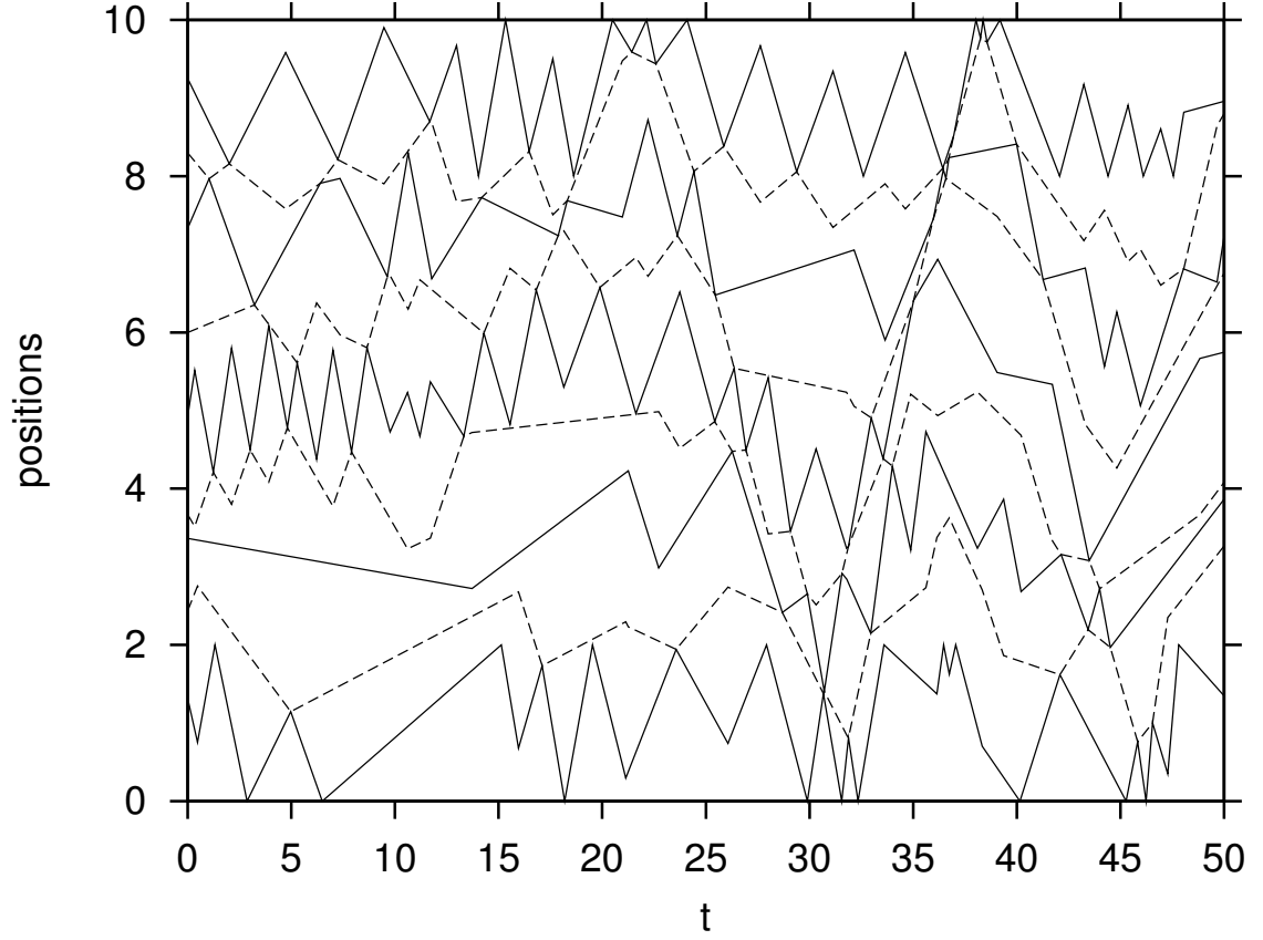
FIG. 4. Typical trajectory of a MC-EBB model with mass ratio m_2/m_1 = 0.382 and size L = 9 . As in Fig.3, the ordinate shws particle positions ( x_n(t) ) where for clarity the odd n particle trajectories are plotted with full lines while the even n trajectories are dashed. The walls at x = 0 and x = 10 act as thermal baths at temperature T = 1 . .
