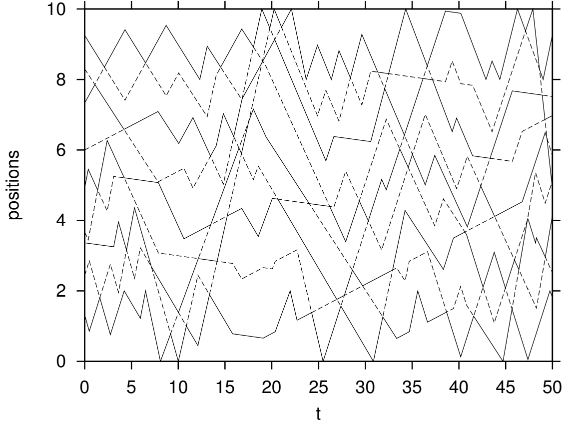
FIG. 3. Typical trajectories of the individual particles in a MC-PIBB model with constant unit masses and size L = 9 . The ordinate shows particle positions ( x_n(t) ) where for clarity the odd n particle trajectories are plotted with full lines while the even n trajectories are dashed. The walls at x = 0 and x = 10 act as thermal baths at temperature T = 1 .
