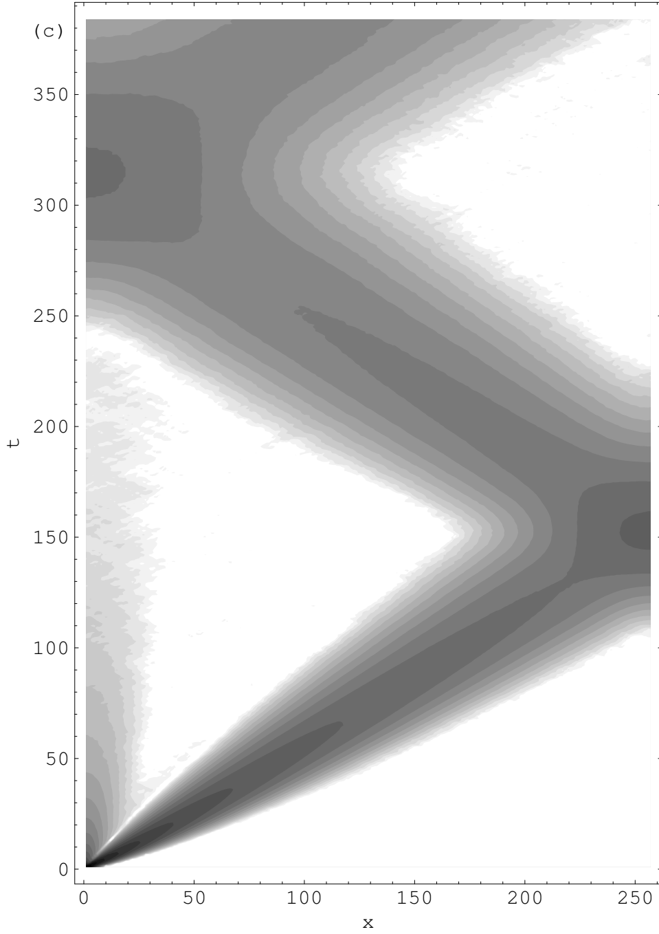
FIG. 9. The spatiotemporal correlation function S(m, t) = \langle j_m(t) j_0(0) \rangle_\beta for the same three cases as in Fig.8. Note the apparent ballistic propagation. Regions between contours of equidistantly spaced base- e logarithm \ln S(x = m, t) are shaded with 20 different and uniformly increasing levels of greyiness in the range [-10, 0] .
