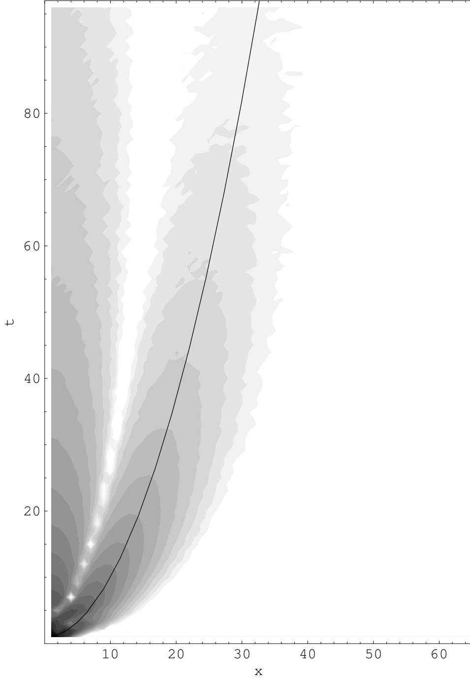
FIG. 16. The spatiotemporal correlation function S(m, t) = \langle j_m(t) j_0(0) \rangle_\beta for the same parameters as in previous Fig.15 and using the same graphical presentation as in Fig.9. Note the apparent diffusive propagation. The superimosed full curve is t = 0.09x^2 .
