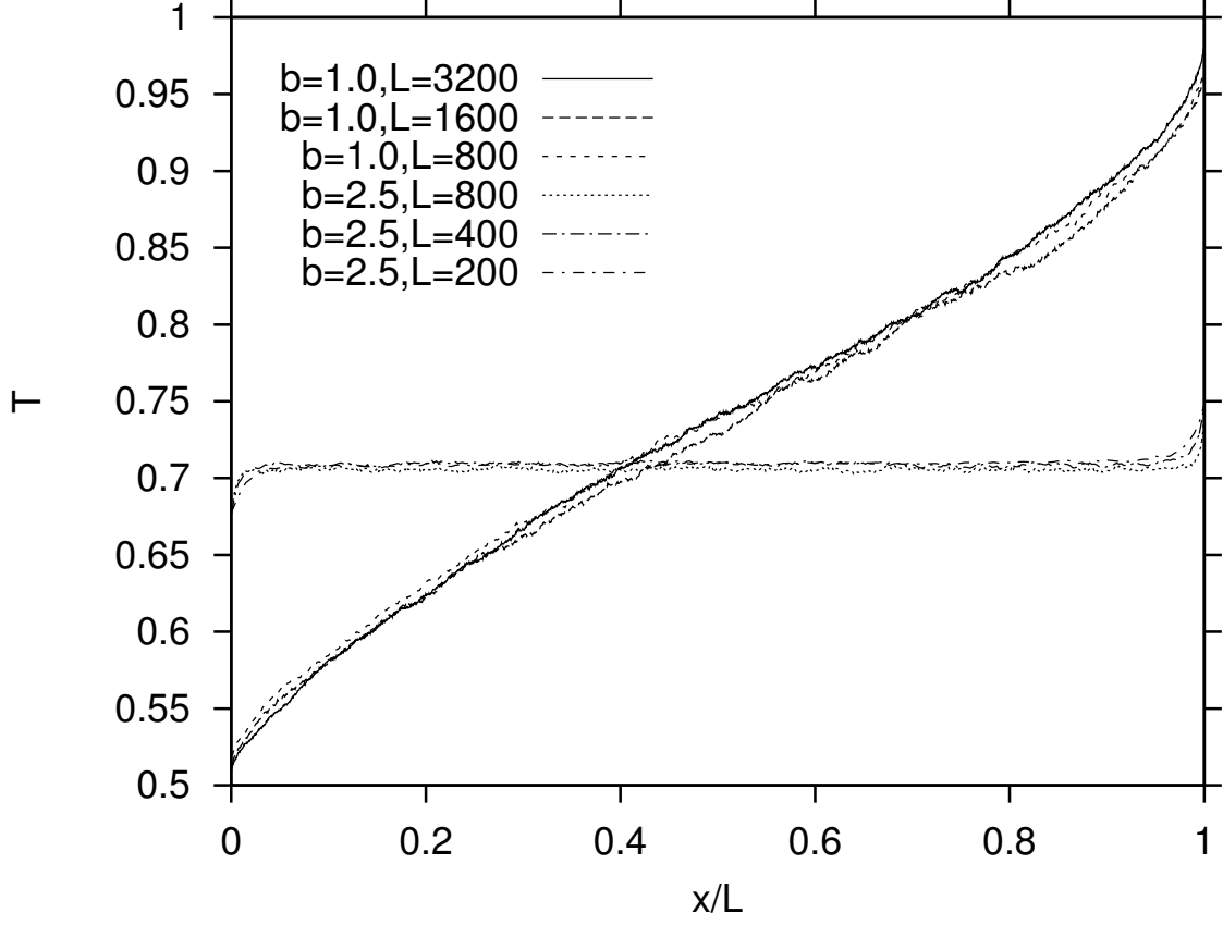
FIG. 5. Scaling of temperature profiles (temperature vs. x/N for different system sizes N ) in a MC-PIBB model with thermal baths at temperatures T_L = 0.5, T_R = 1.0 . The triple of steep curves refers to a system with symmetric interparticle potential b = 1.0 (so that the pressure vanishes), while the triple of horizontal curves (at T = \sqrt{T_L T_R} , so zero temperature gradient over the bulk of the chain) refers to b = 2.5 (and a non-vanishing pressure).
