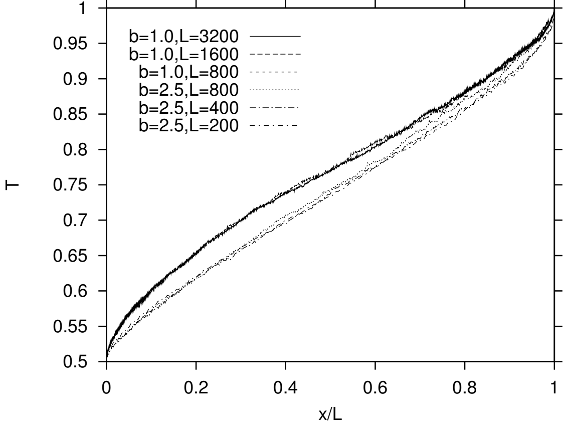
FIG. 6. Scaling of temperature profiles (temperature vs. x/N for different system sizes N ) in a MC-EBB model with mass ratio m_2/m_1 = 0.382 . All other parameters are the same as in Fig.5. Note that here a nonvanishing temperature gradient is established even in the non-symmetric case b = 2.5 with nonvanishing pressure.
