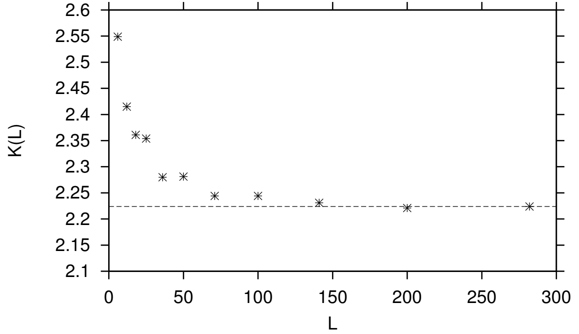
FIG. 14. Convergence of the thermal conductivity \kappa(L) to its L -independent asymptotic value for the MNC-PIBB model. In the simulations, T_L = 1 , and T_R = 2 .
