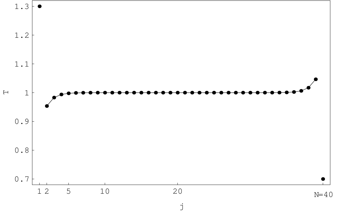
FIG. 1. Temperature profile for the linear optical chain with the parameter \tilde{\nu} = 0.25 and with reservoir temperatures T_L = 1.3, T_R = 0.7 . The size of the lattice here is N = 40 . As discussed in the text, this profile is the same as for the linear acoustic chain discussed in Ref. (11)
