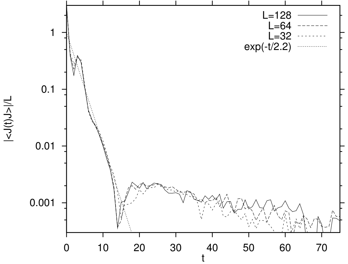
FIG. 15. The magnitude of the current autocorrelation function |\langle J(t)J \rangle|/L (at temperature T = 1 ) for the MNC-PIBB model with periodic boundary conditions for different system sizes.
