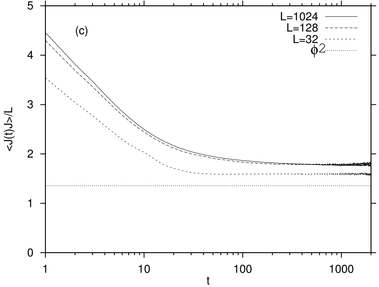
FIG. 8. The current-current temporal autocorrelation function \langle J(t)J \rangle_\beta / L (at temperature T = 1 ) for: (a) the pseudointegrable ( m_2/m_1 = 1 ) momentum-conserving bing-bang model with periodic boundary conditions and vanishing pressure, b = 1.0 ; (b) the ergodic momentum-conserving bing-bang lattice ( m_2/m_1 = 0.382 ) with vanishing pressure, b = 1.0 ; and (c) the ergodic momentum-conserving lattice with non-vanishing pressure b = 2.5 . In each case, three different system sizes are shown. Note that the dotted line in (c) indicates the lower bound from the theorem from section IV.
