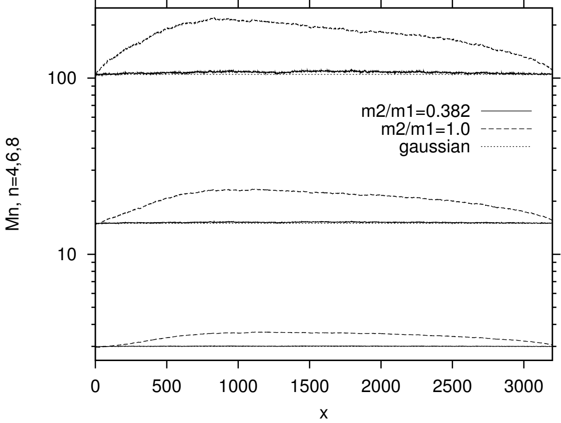
FIG. 11. Moments of the velocity distributions M_{2n}(m) = \langle p_m^{2n} \rangle_\beta / \langle p_m^2 \rangle_\beta^n for n = 4, 6 , and 8 for two different momentum conserving bing-bang lattices of size L = 3200 with T_L = 0.5, T_R = 1.0 . The results for the EBB model (with m_2/m_1 = 0.382 , plotted as solid lines) are essentially indistinguishable from those of the Gaussian model ( M_n = (2n - 1)!! ), plotted as dotted lines), showing that local thermal equilibrium is established in the MC-EBB model, whereas the results for the MC-PIBB model (dashed lines) deviate substantially from the Gaussian model, showing that local thermal equilibrium is not established, as anticipated by the heuristic argument presented in the text.
